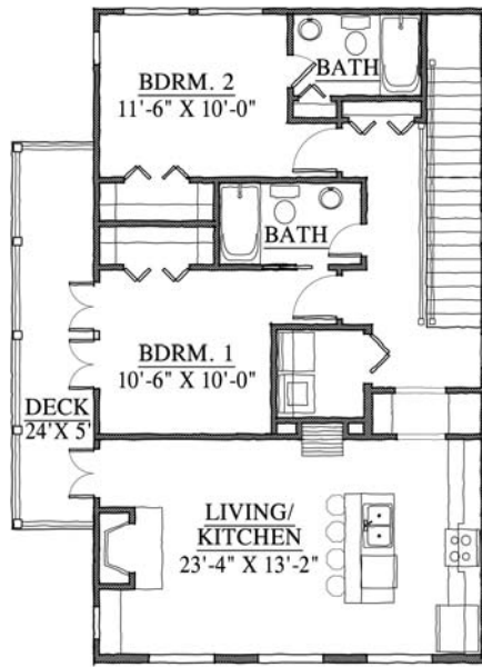
Second Floor Plan 960 Square Feet
