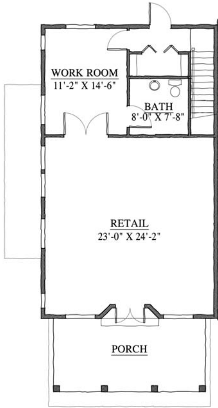
First Floor Plan 960 Square Feet
