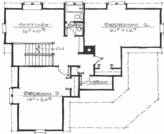
Second Floor Plan 1151 Square Feet
