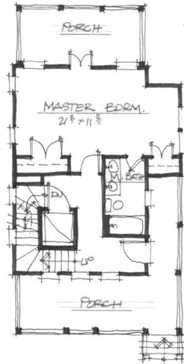
First Floor Plan 498 Square Feet
