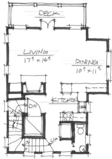
Second Floor Plan 450 Square Feet
