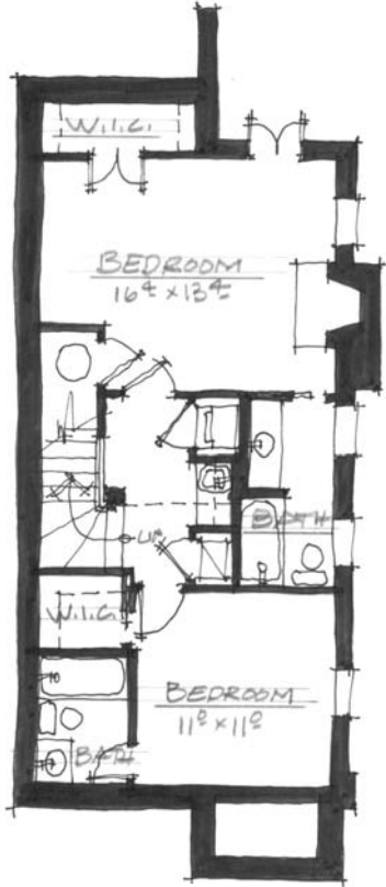
Ground Floor Plan 643 Square Feet
