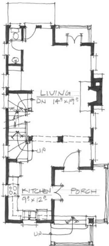
First Floor Plan 556 Square Feet
