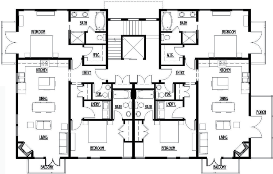
SECOND / THIRD FLOOR PLAN 1,177 Finished Square Feet Per Flat
