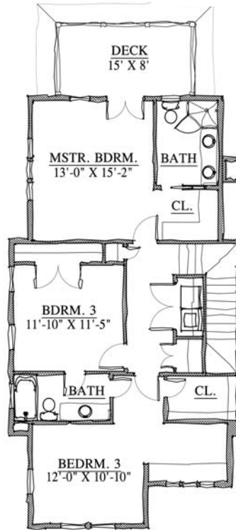
Upper Floor Plan 974 Square Feet
